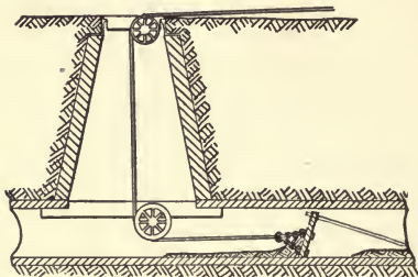
FIG. 36.—METHOD OF USING CLEANING-DISK.
